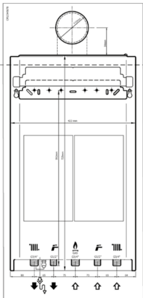
Figure 1 Installation scheme
